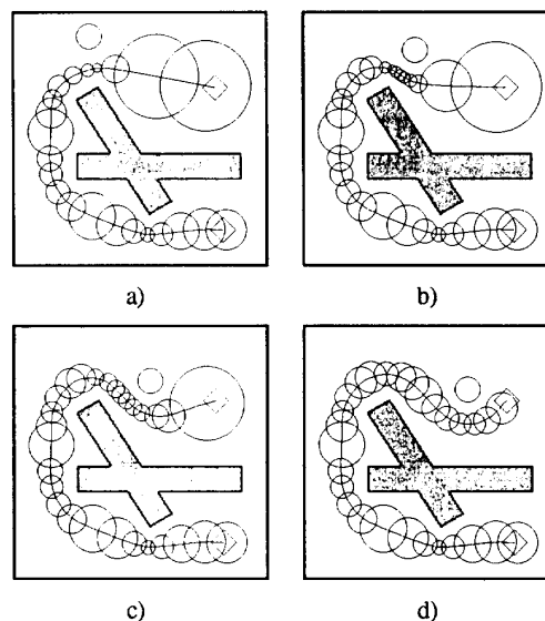
Figure 4. As an obstacle moves, the bubbles also move to minimize the force on the elastic band. If needed, bubbles are inserted and deleted to maintain a collision free path.
